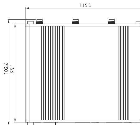
Communications Module - Side
